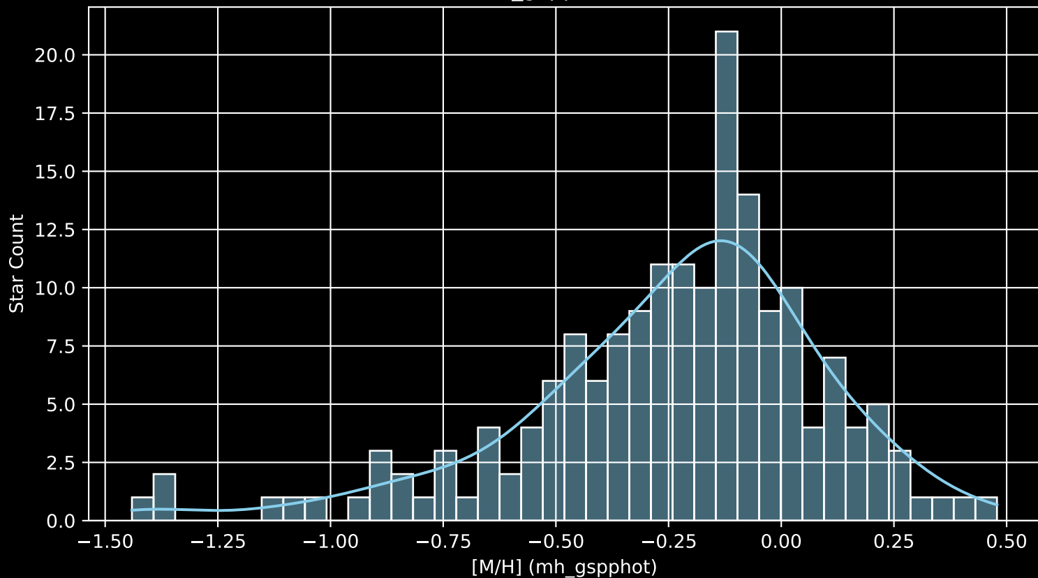
APOGEE DR17 Field: [266-26-O TESS [M/H] (mh_gspphot) (n= 177)
