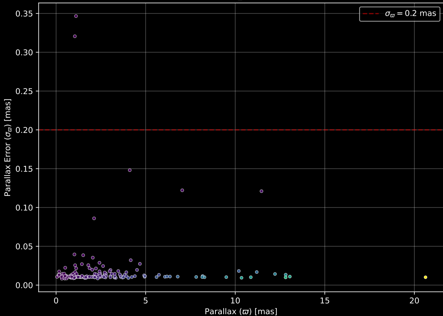
APOGEE DR17 Field: [266-26-O_TESS] Parallax Quality (n= 179)
