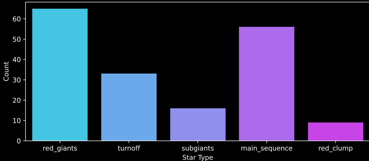
APOGEE DR17 Field: [266-26-O_TESS] Count plot of Star Type
