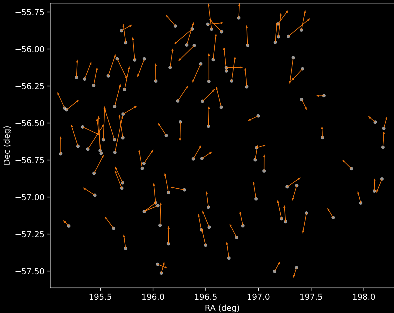
APOGEE DR17 Cluster 2 Proper Motion Vectors (n=105)
