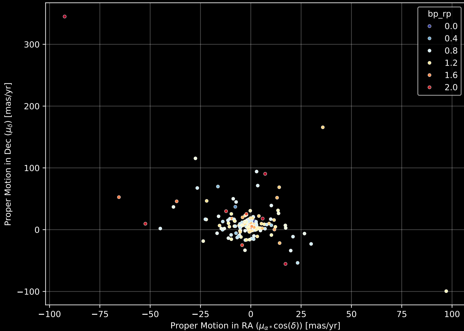
APOGEE DR17 Field: [266-26-O_TESS] Proper Motion Diagram (n= 179)
