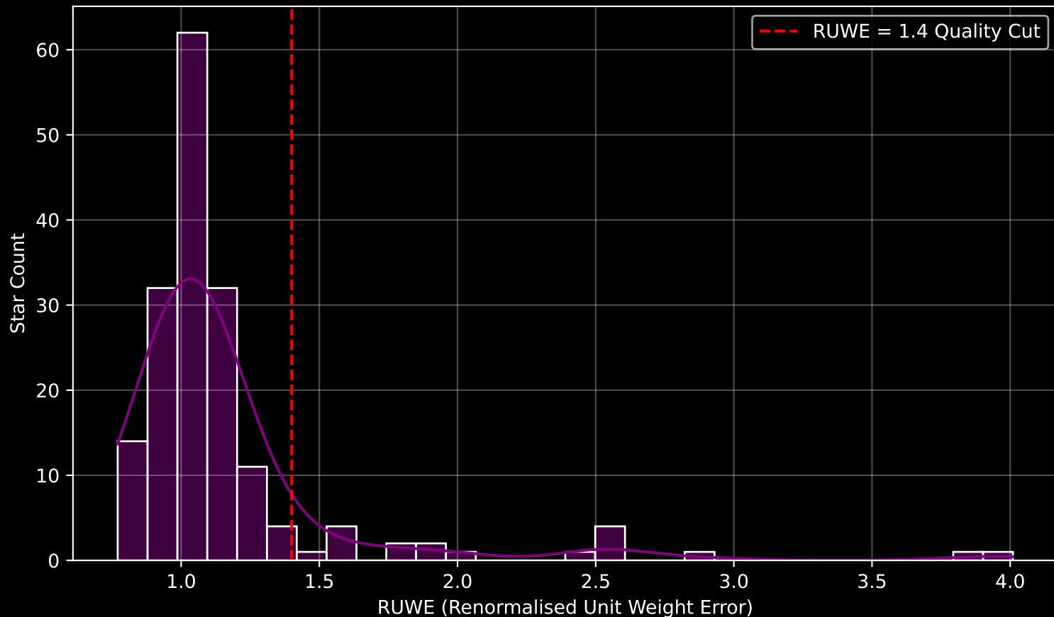
GAPOGEE DR17 Field [266-26-O_TESS] RUWE Distribution (n= 173)
