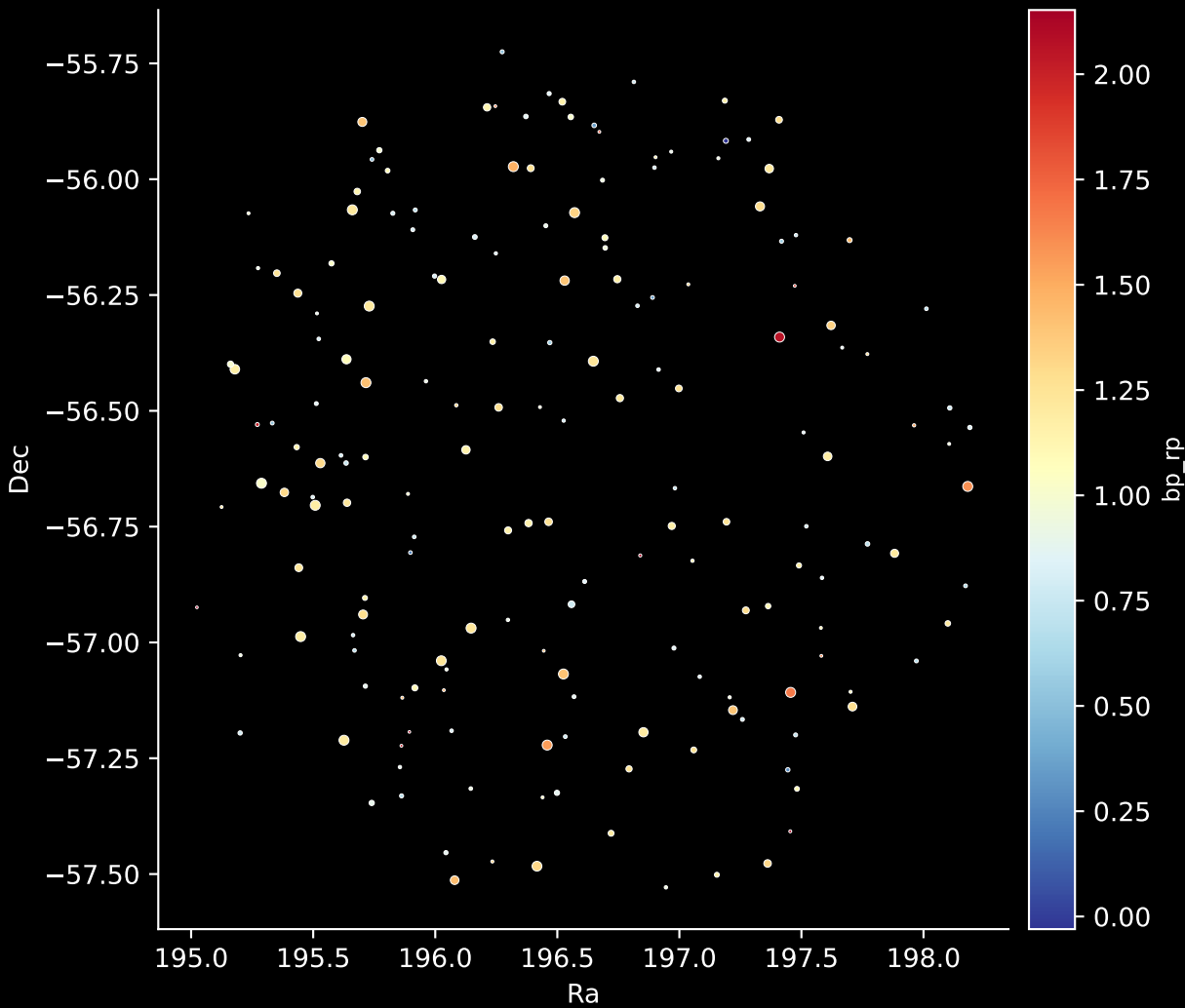
APOGEE DR17 Field: [266-26-O_TESS] Stars: 179
